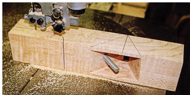
Shape the plane. Cut the raze section and coffin sides on the band saw.
